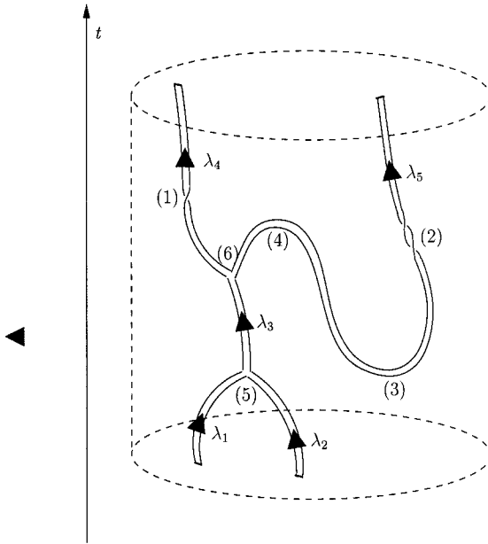
Fig. 1. A Feynman diagram or ribbon graph for some sources. One can recognize (1) a self-twist, (2) a double self-twist, (3) a pair production, (4) a pair annihilation, (5) two sources that fuse into one, and (6) a source that splits in two.
