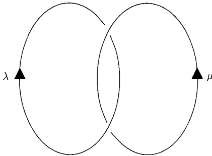
Fig. 4. The link whose link invariant in the three sphere S^3 equals S_{\lambda\mu} .
