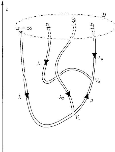
Fig. 2. A ribbon graph for a state in \mathcal{H}_{z, \bar{\lambda}}[v_\lambda] .
