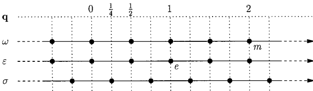
Fig. 5. Physically realized representations for \mathcal{C} = \text{Vir}_1 ; e marks the electron representation, m a multi-electron representation and \bullet the representations that fulfill (63) and hence appear in the theory.
