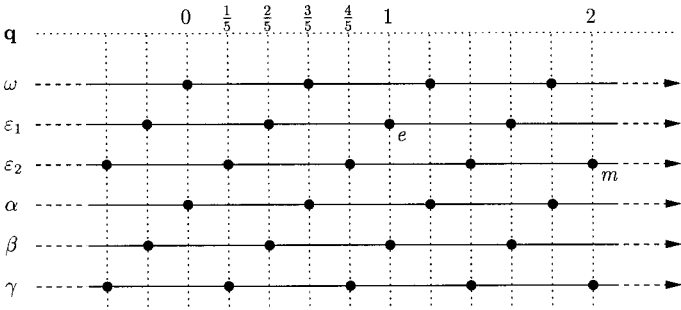
Fig. 6. Representations for \mathcal{C} = W_3 ; e marks the electron representation, m a multi-electron representation and \bullet the representations that fulfill (63) and hence can appear in the theory.
